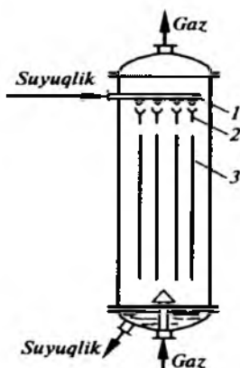
7- rasm. Yupqa qatlamli absorber: Odatda, nasadkalar qatlami 1 – quvur; 2 – taqsimlash moslamasi; 3 – tekis parallel nasadka.
