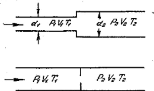
10.9 – rasm. Joule-Tomson effektiga tegishli gaz harakati tasviri.
