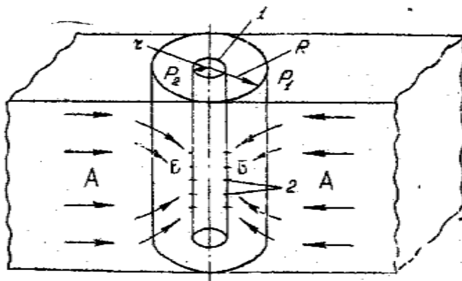
2.5 - rasm. Radial oqimda o'tkazuvchanlikni aniqlash
